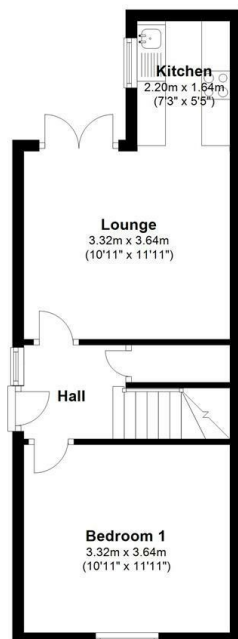
Ground Floor Approx. 34.7 sq. metres (373.6 sq. feet)
